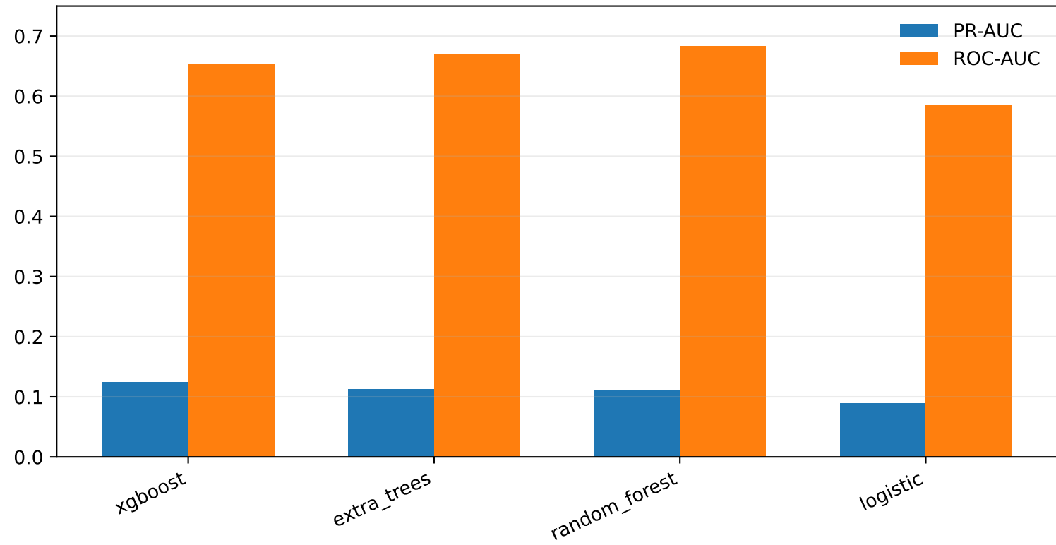
Grouped Cross-Validated Model Ranking
